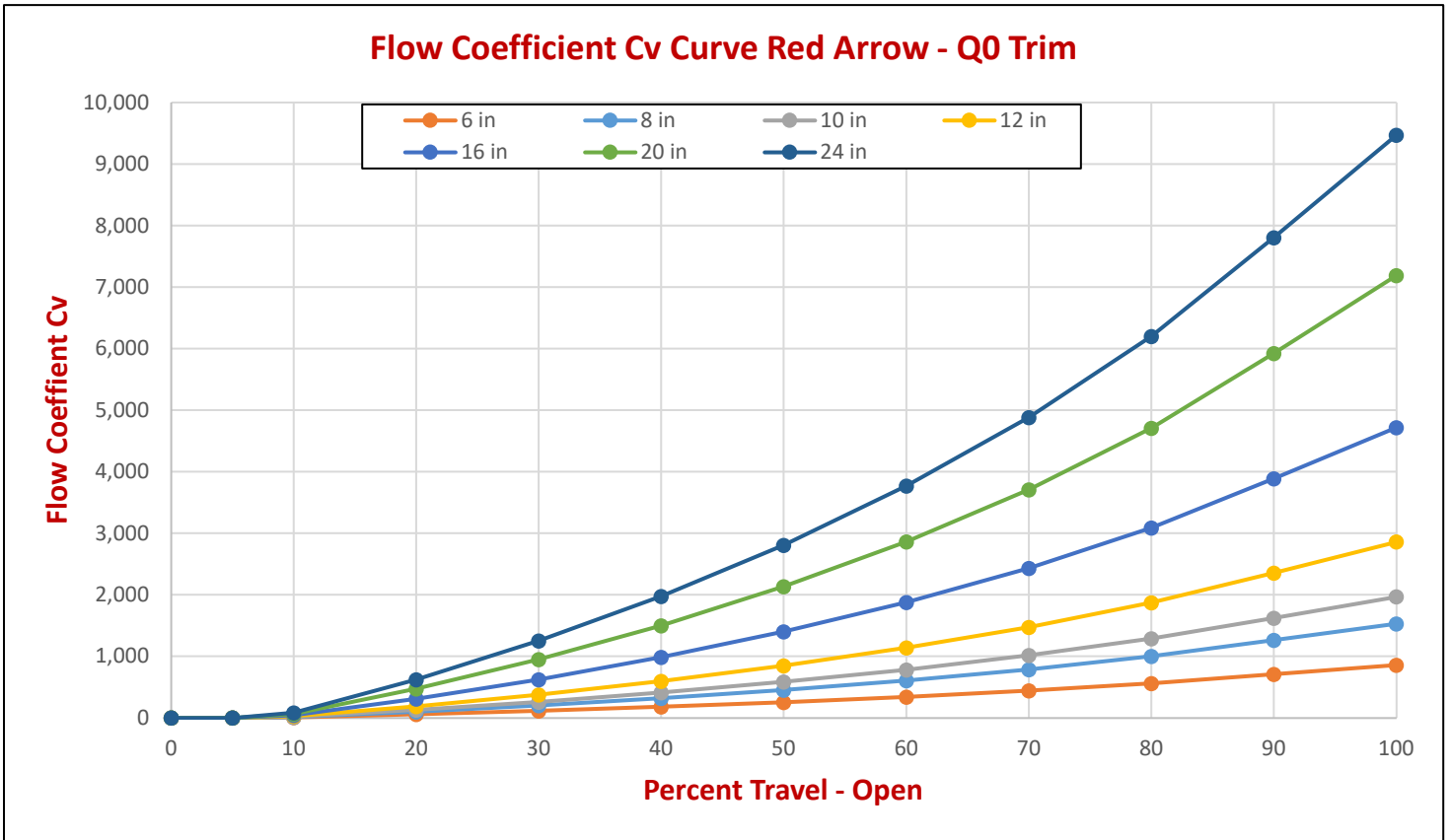
Figure 2.0 - Flow Profile Curve Red Arrow - Q0 Trim
