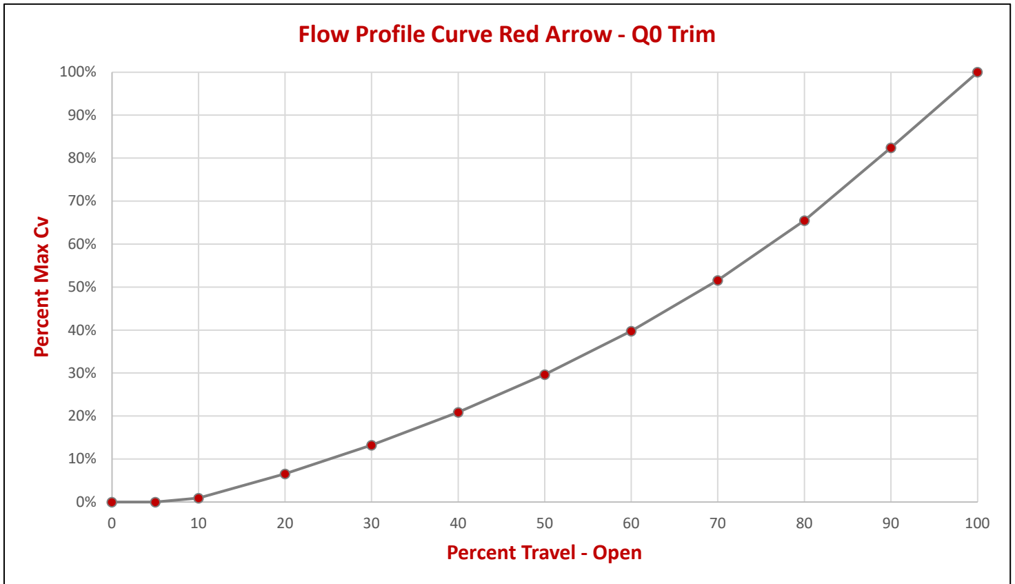
Figure 1.0 - Flow Profile Curve Red Arrow - Q0 Trim
