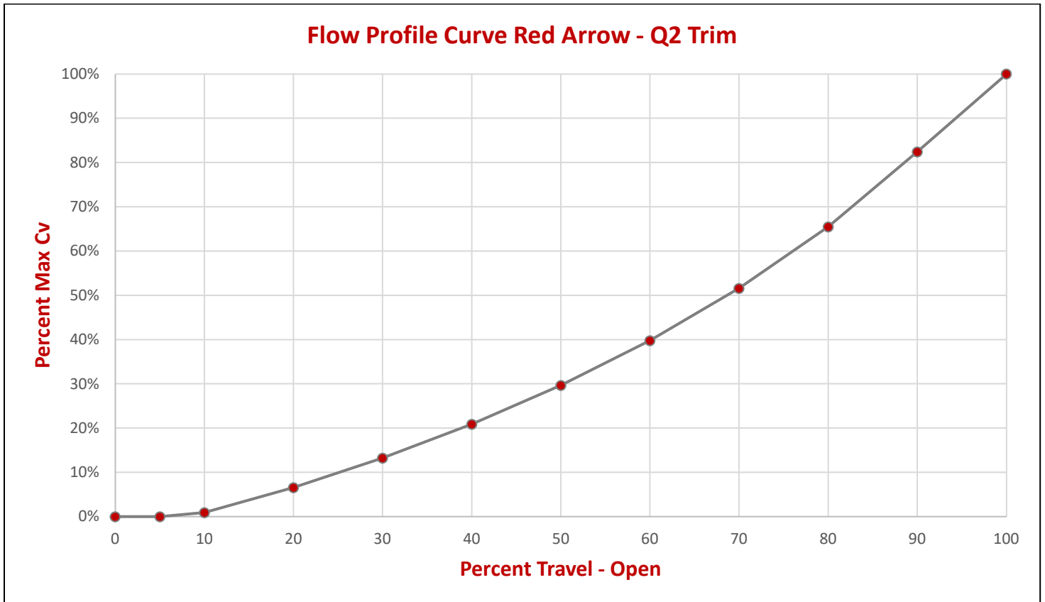
Figure 1.0 - Flow Profile Curve Red Arrow – Q2 Trim
