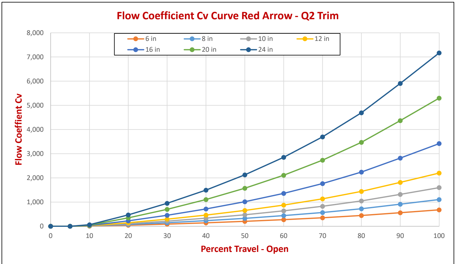
Figure 2.0 - Flow Profile Curve Red Arrow – Q2 Trim
